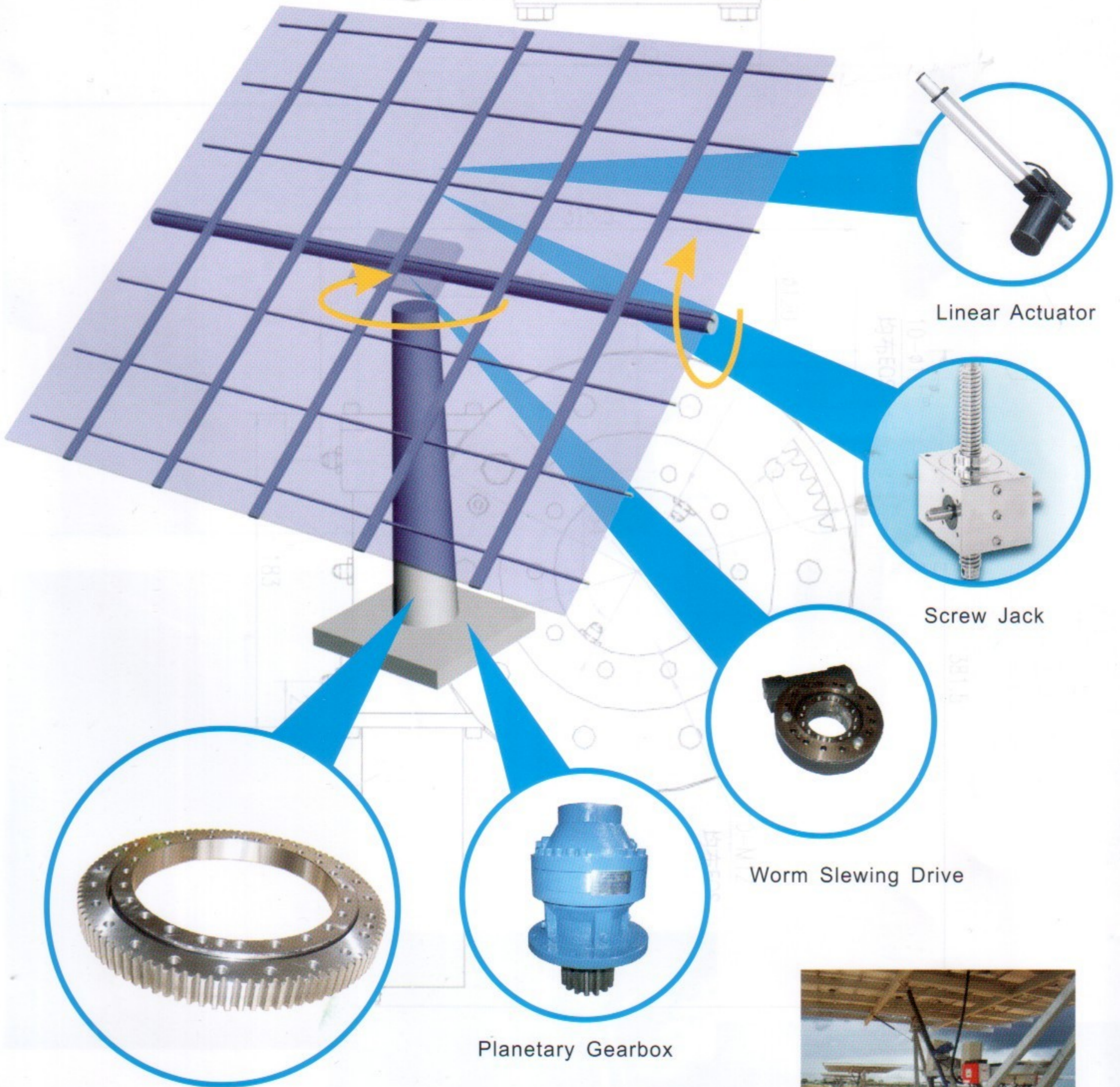
Slewing Bearing
